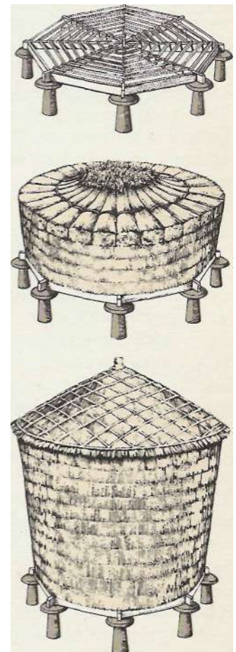
A circular corn stack Lay a base of sheaves with their butts outwards, and build up keeping the centre high. Pull inwards when you reach the leaves and let them overhang slightly so the rain runs off. Use rat-proof staddle stones to keep your stack off the ground, and you will keep out damp as well as rats.
