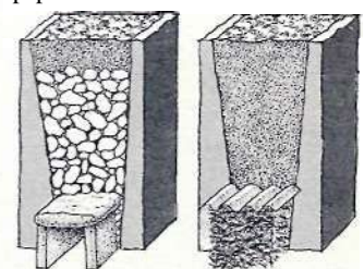
Stone culvert drain
