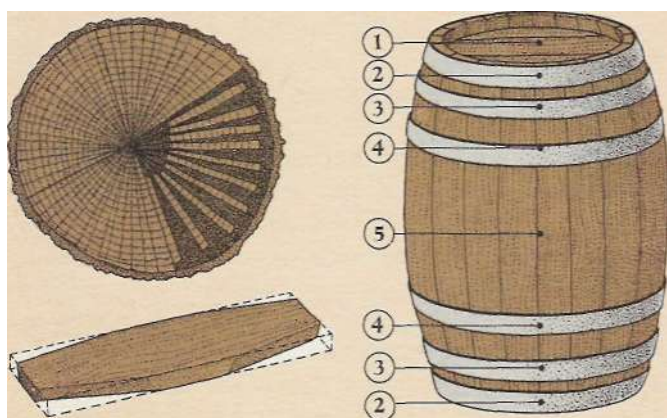
The parts of a barrel
