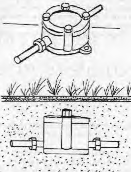
Figure 97. Geophone.
