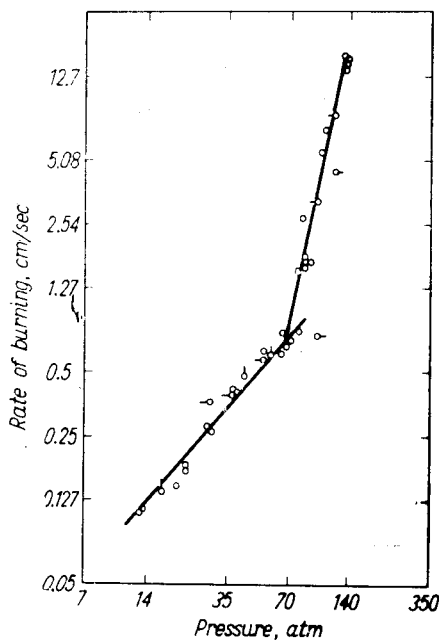
FIG. 78. The relation between the rate of burning of the stoichiometric mixture of 2-nitropropane with nitric acid and the pressure (according to Tait, A. E. Whittaker and Williams [23]).
