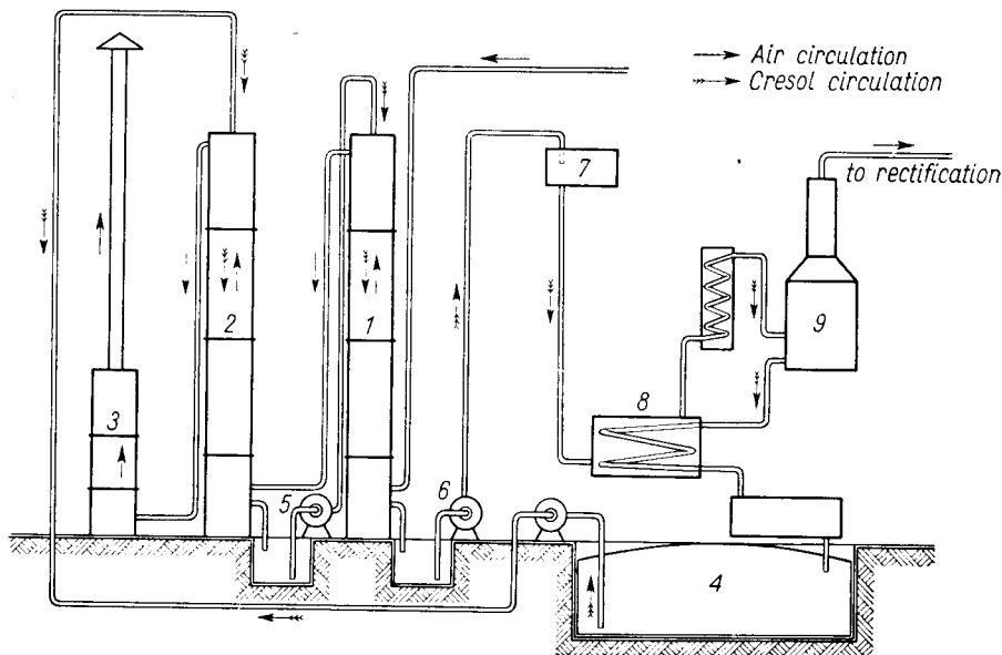
FIG. 225. Schematic view of an installation for the absorption of solvent with cresol (Brégeat method).
