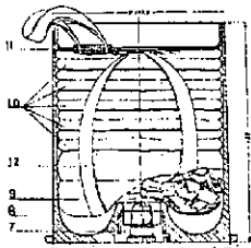
Cartridge with Igniter Tube
