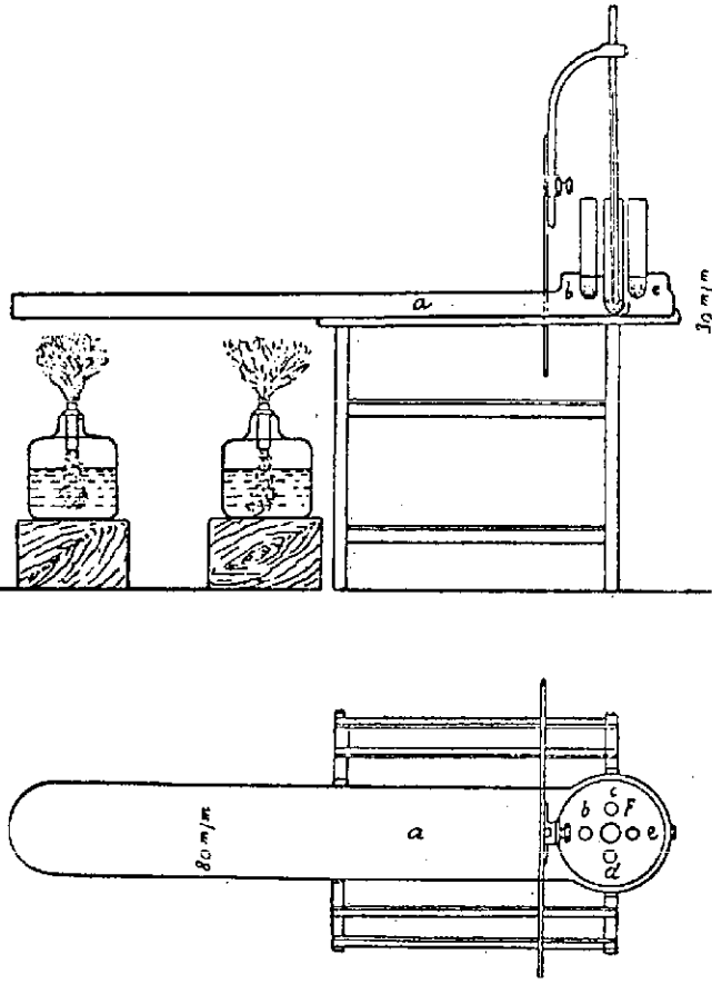
Fig 83. Apparatus for Determining the Temperature of Ignition
