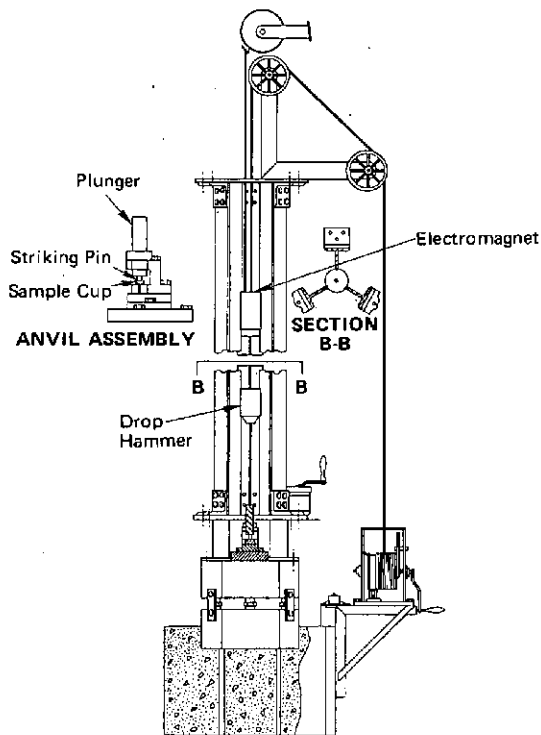
Fig 4. Impact Apparatus Showing Anvil-striking Pin Assembly
