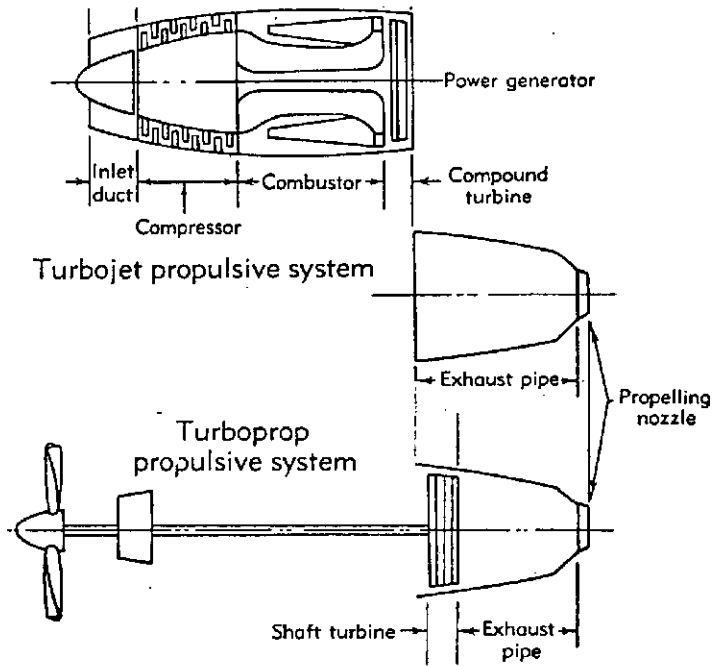
Fig 2. Comparison of Turbojet & Turboprop Engines
