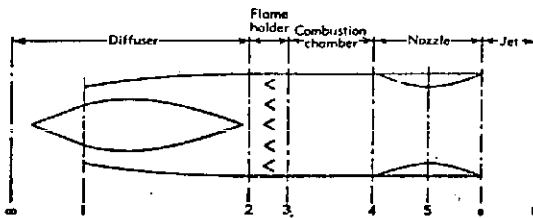
Fig 3. Schematic of ramjet engine
