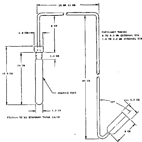
FIGURE 2 Apparatus for 100°C vacuum stability test
