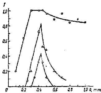
Fig 13. Explosion frequency vs charge thickness in the case of HMX for various impact energies
