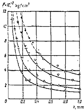
Fig 9. Average pressures upon fracture ( P_{ult} —solid curves) and upon explosion ( P_{ex} —dashed curves) vs charge thickness of HMX (○), RDX (▽), Tetryl (△) and TNT (□)
