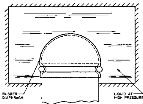
Fig 7 Hydrostatic Press Principle
