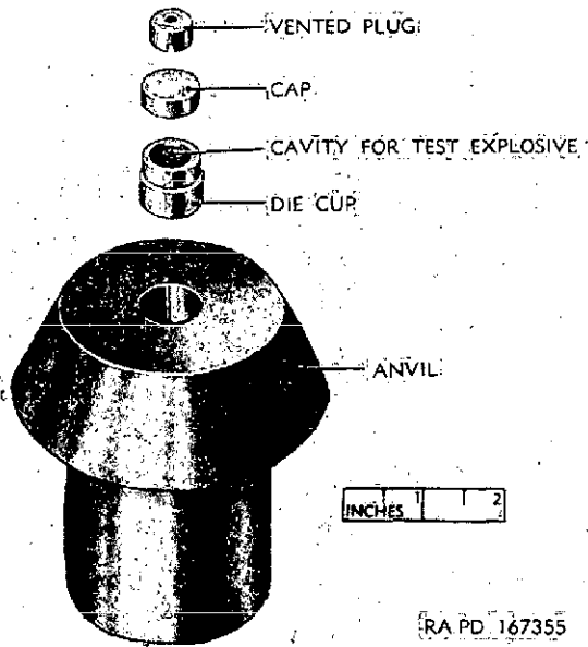
Fig 5-2. Parts of Picatinny Arsenal Impact Test Apparatus
