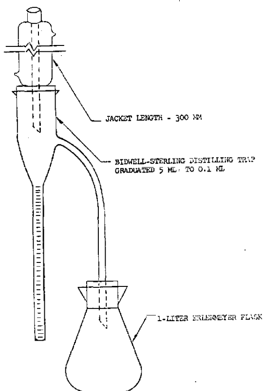
FIGURE 1 Moisture content apparatus
