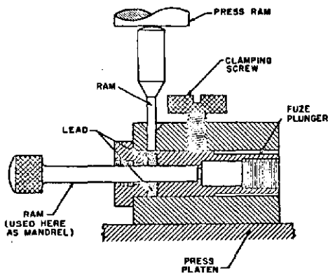
Fig 4 Tool for Direct Loading of Component
