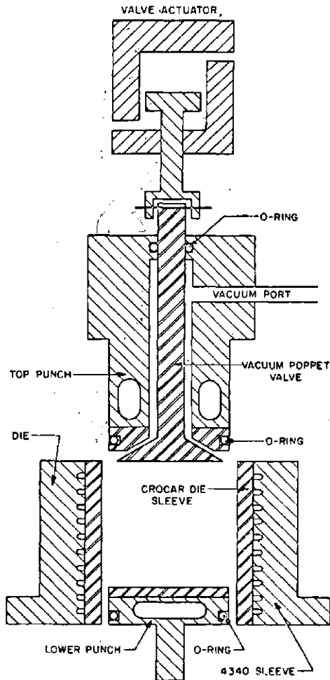
Fig 6 Vacuum Pressing Apparatus
