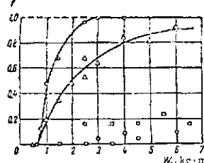
Fig 12. Explosion frequency vs impact energy for Tetryl ( \square ) and RDX ( \triangle ) for charges 0.4mm thick and for HMX ( \circ ) charges 0.5mm thick
