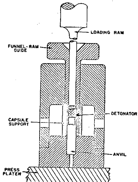
Fig 3 Detonator Loading Tool
