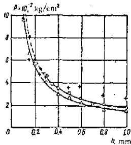
Fig 10. Average pressures P_{ult} and P_{ex} vs charge thickness for PETN (○) and Trinitrophenol (△) Points marked + refer to Dina
