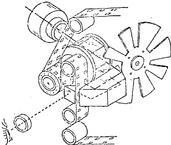
Mechanism of rotating prism Photec camera
