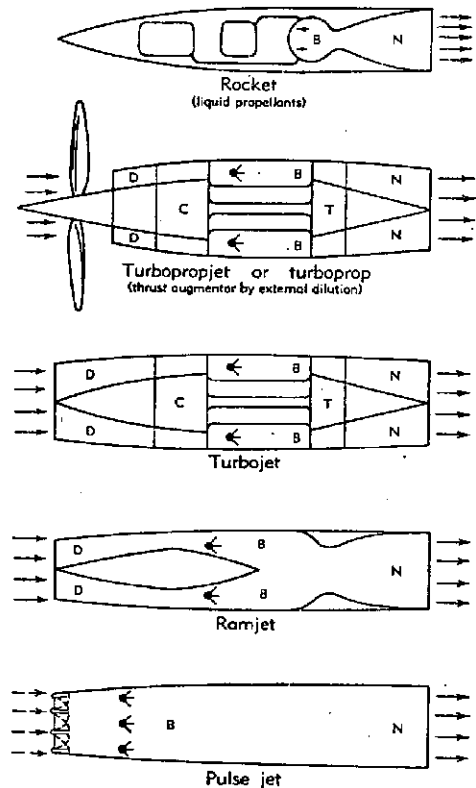
Fig 1. Types of Jet Propulsion Engines
