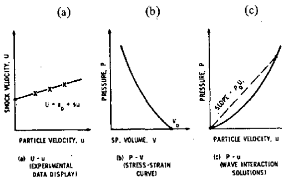
Fig 2 Alternative Hugoniot curves
