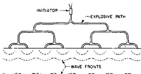
Line Wave Generator of the Manifold Type
