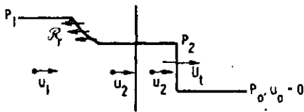
Fig 3 Transmission of a plane shock wave into a material of lower impedance
