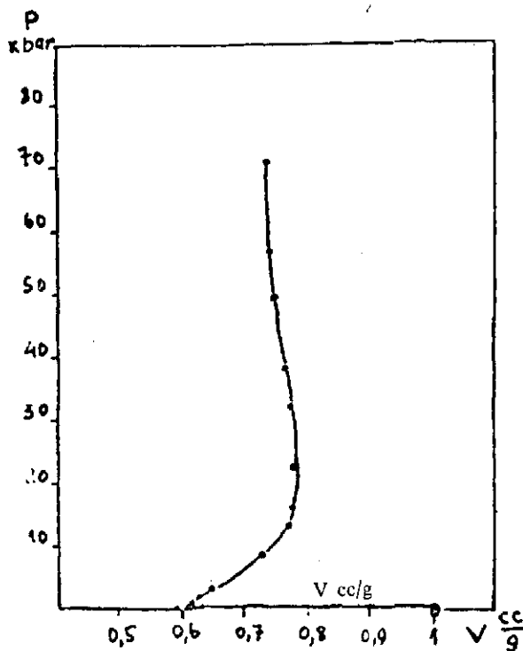
Fig 7 P-V Hugoniot for 1 g/cc TNT
