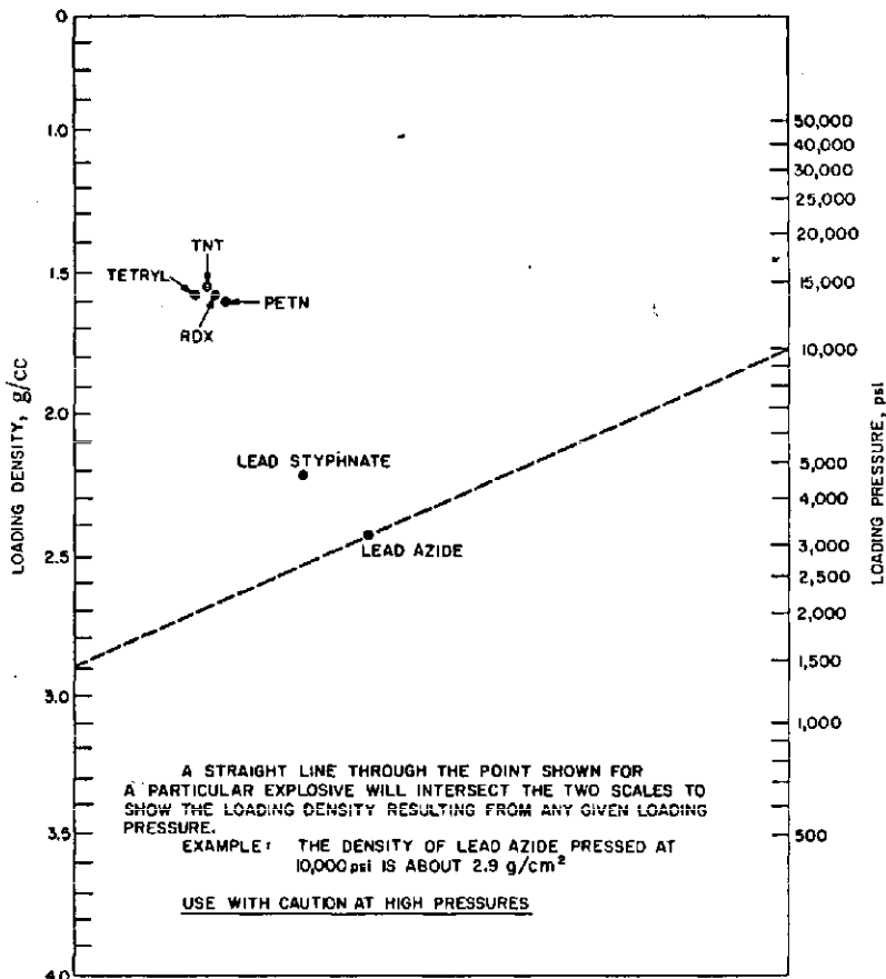
Fig 5 Nomograph of Loading Pressure and Density
