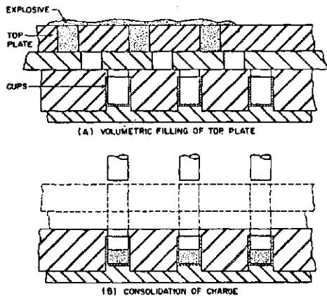
Fig 2 Charging Plate Loading
