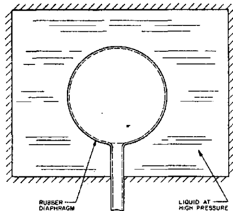
Fig 8 Isostatic Press Principle
