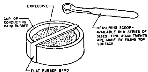
Fig 1 Scoop Loading
