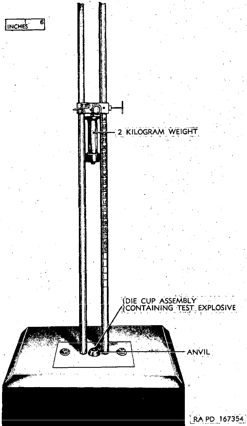
Fig 5-1. Picatinny Arsenal Impact Test Apparatus
