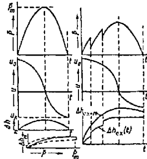
Fig 8. Interpretation of oscilloscope traces of pressure pulses
