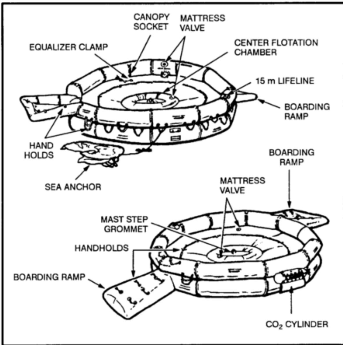
Figure 16-15. Twenty-man raft.
