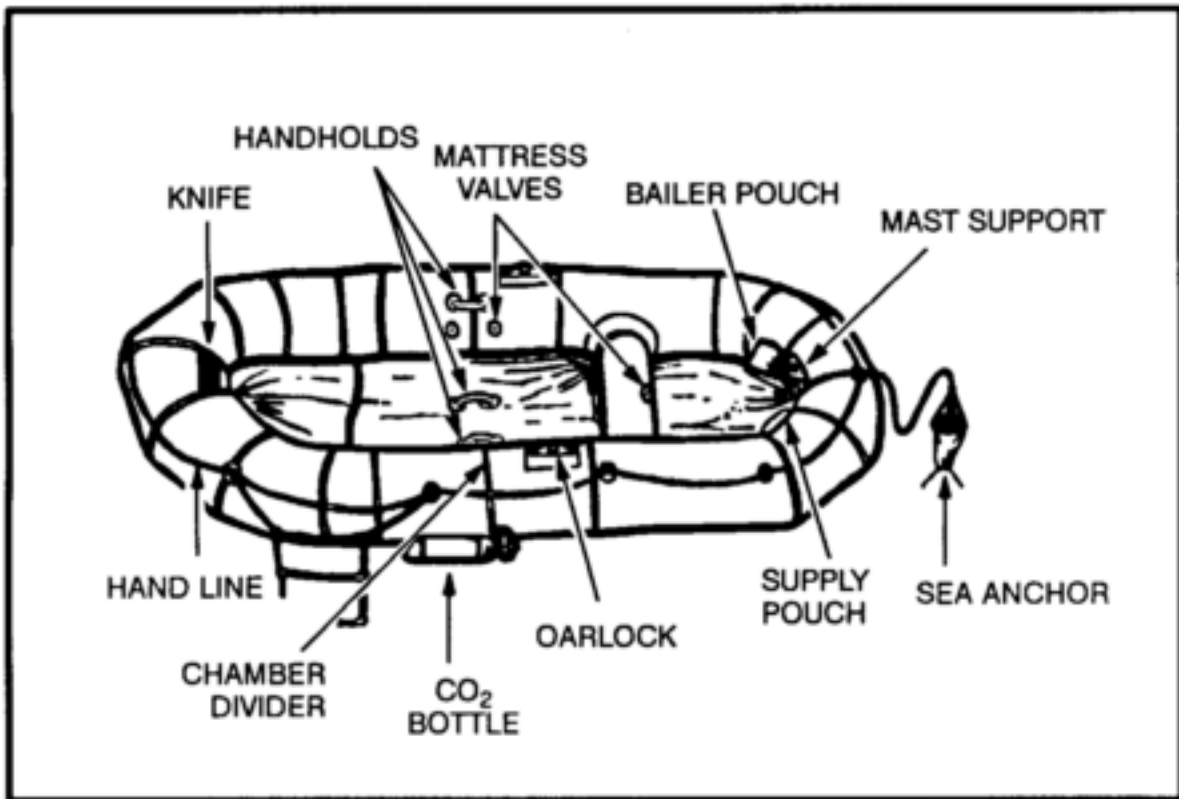
Figure 16-12. Seven-man raft.
