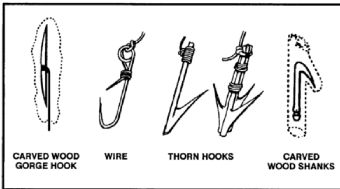
Figure 8-17. Improvised fishhooks.
